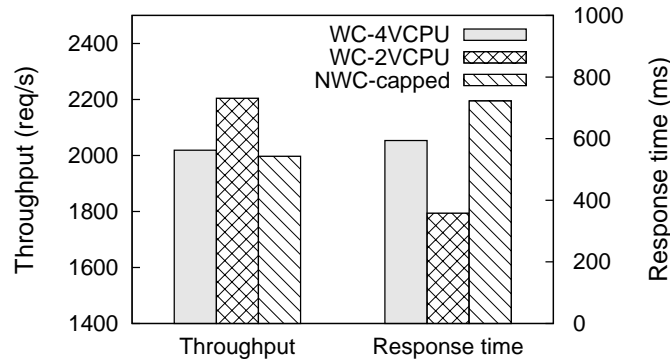
Figure 6.1: Performance of TPC-W under different CPU allocation modes.
