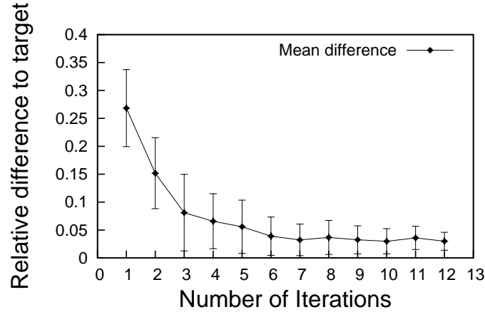
Figure 5.10: Performance deviation during re-configuration.
