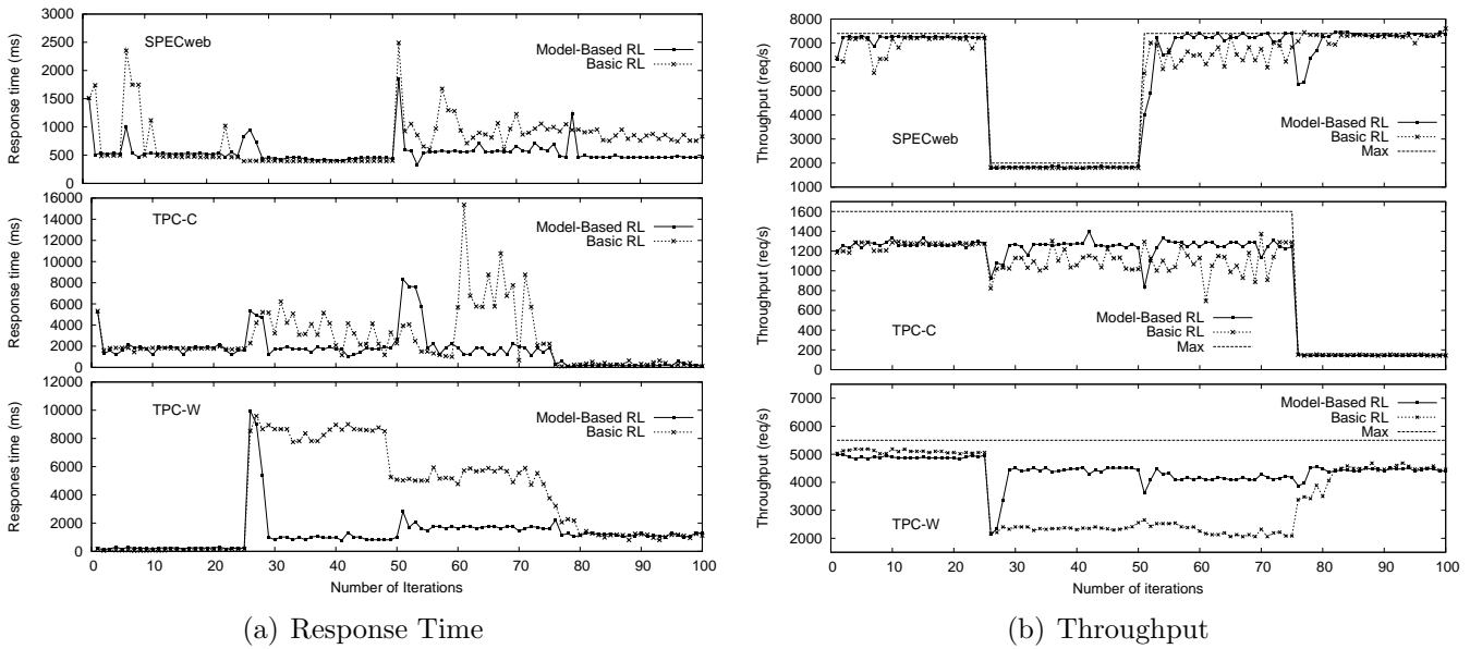
Figure 5.11: Performance of VCONF with heterogeneous applications.
