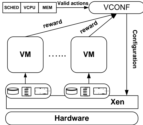
Figure 5.4: The organization of VCONF.
