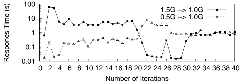
Figure 5.2: Delayed effect in memory reconfiguration.
