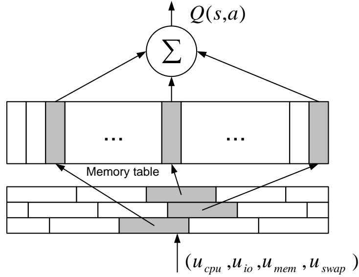
Figure 6.3: CMAC-based Q table.
